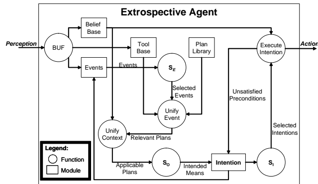
Fig. 1. The extrospective agent architecture
